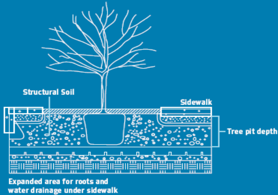
Improved Tree Pit Design
